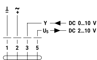
TF230-S / TF24-S
