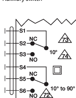
Auxiliary Switch
