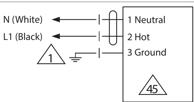
120 VAC
