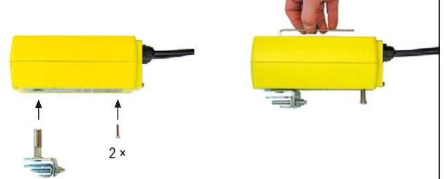
1. Pre-assemble mounting clamp
