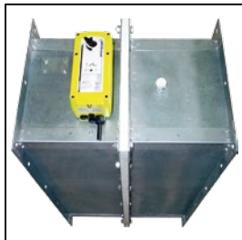
Fire damper
