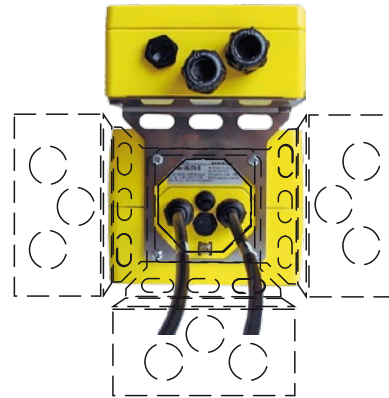
Terminal box mounted beside the actuator
